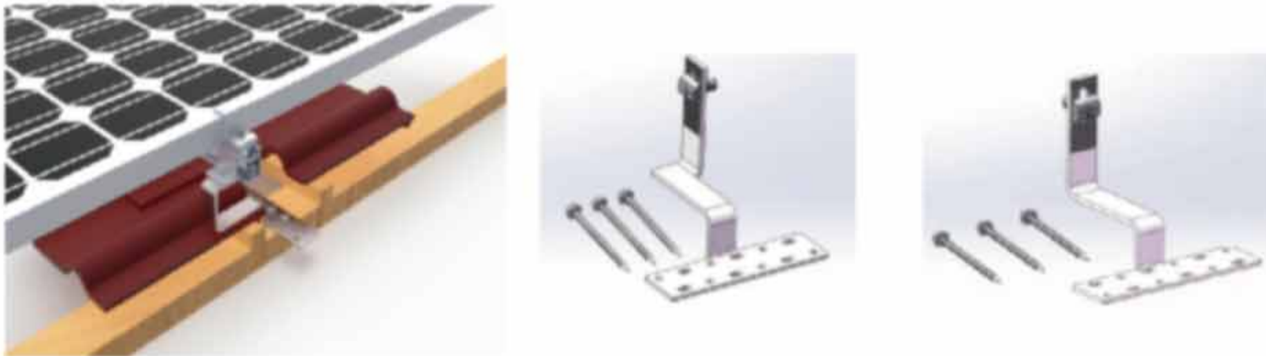
JS-R-09 -1 Roman Tile Roof Solar Mounting System
